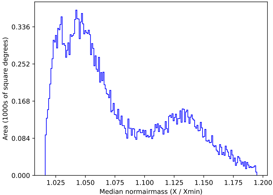
too_elab_r128_d2_griz_v3.4_10yrs All sky r band: Median normairmass
