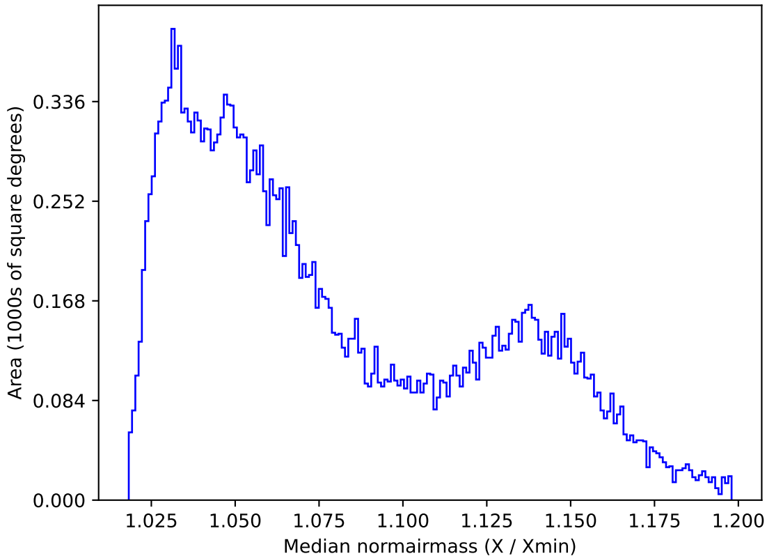
too_elab_r128_d2_griz_v3.4_10yrs All sky i band: Median normairmass
