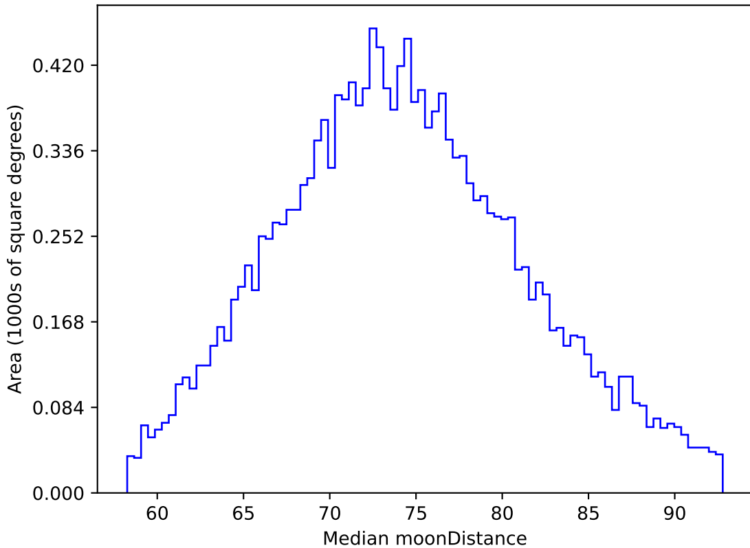
too_elab_r128_d2_griz_v3.4_10yrs WFD z band: Median moonDistance
