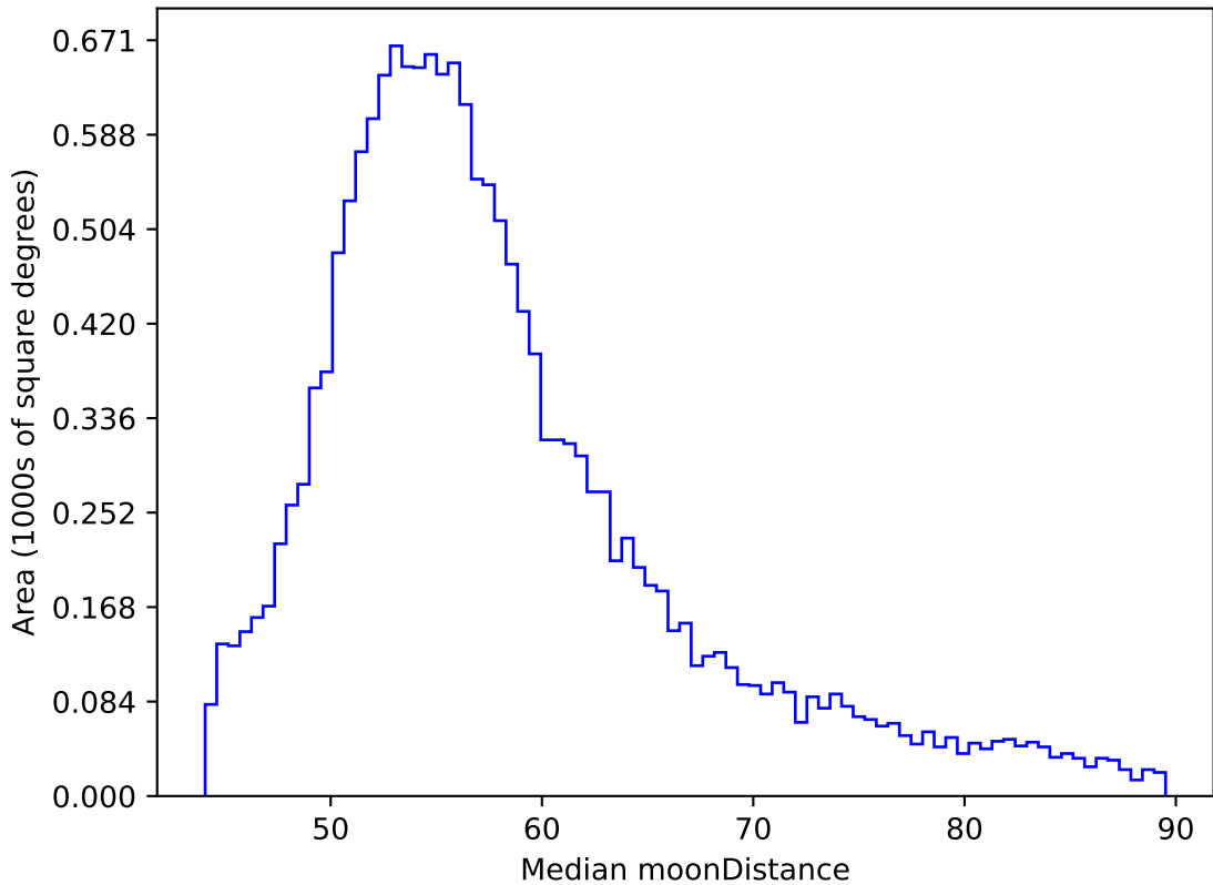
too_elab_r128_d2_griz_v3.4_10yrs WFD y band: Median moonDistance
