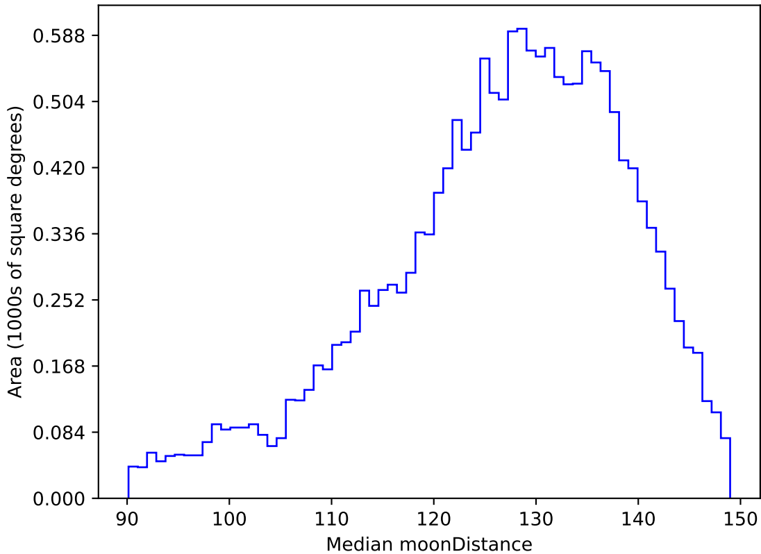
too_elab_r128_d2_griz_v3.4_10yrs WFD u band: Median moonDistance
