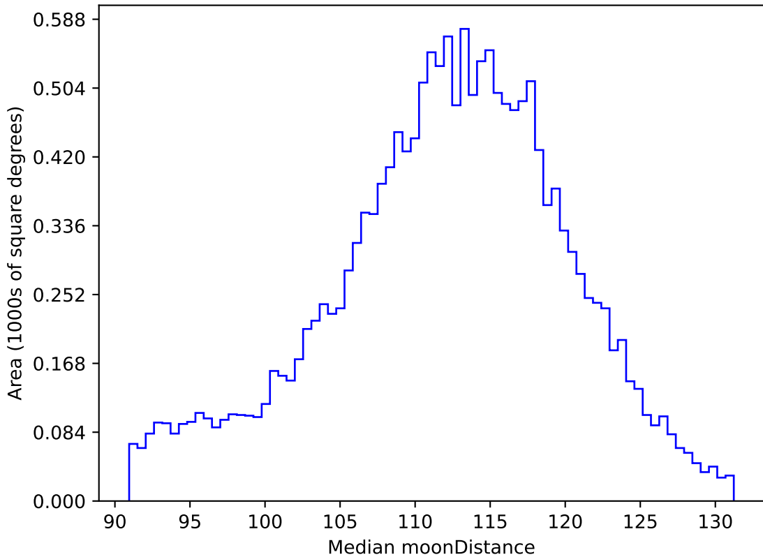
too_elab_r128_d2_griz_v3.4_10yrs WFD r band: Median moonDistance
