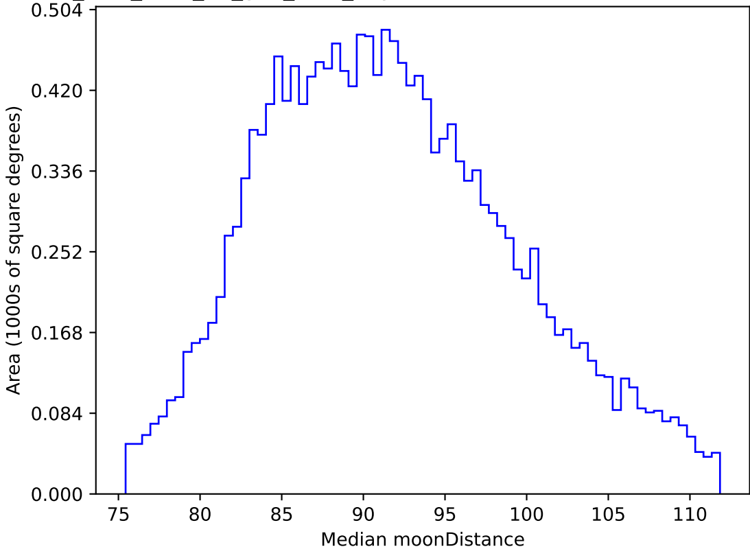
too_elab_r128_d2_griz_v3.4_10yrs WFD i band: Median moonDistance
