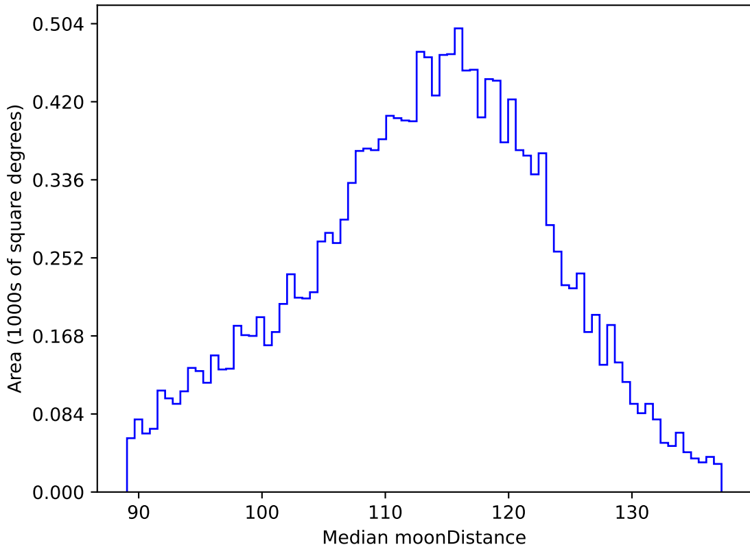
too_elab_r128_d2_griz_v3.4_10yrs WFD g band: Median moonDistance
