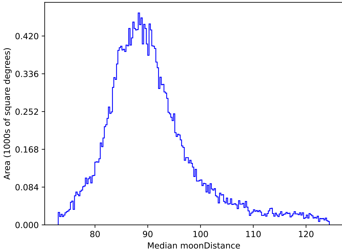
too_elab_r128_d2_griz_v3.4_10yrs All sky all bands: Median moonDistance
