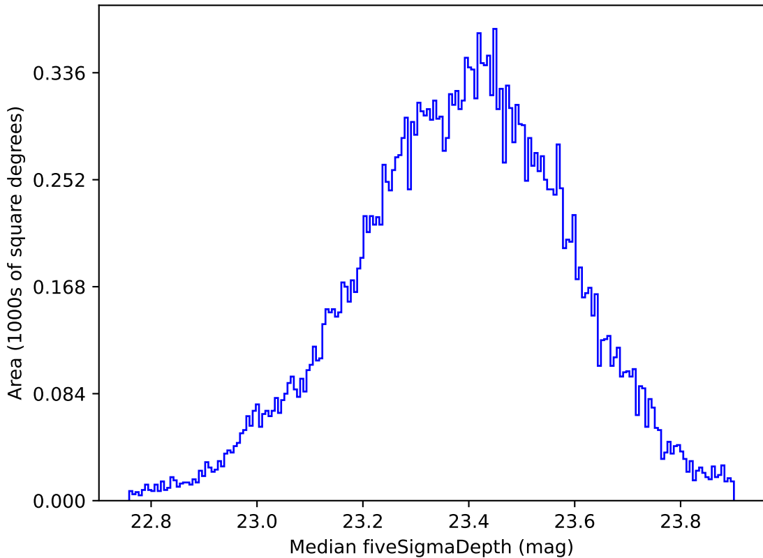
too_elab_r128_d2_griz_v3.4_10yrs Yr 1 all bands: Median fiveSigmaDepth
