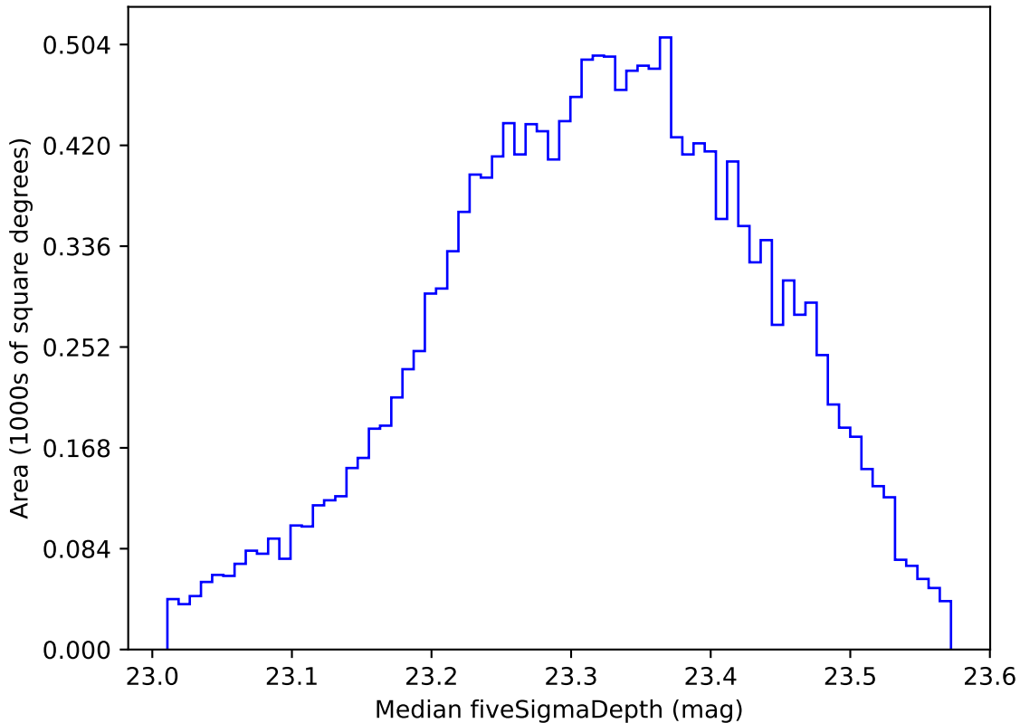
too_elab_r128_d2_griz_v3.4_10yrs WFD all bands: Median fiveSigmaDepth
