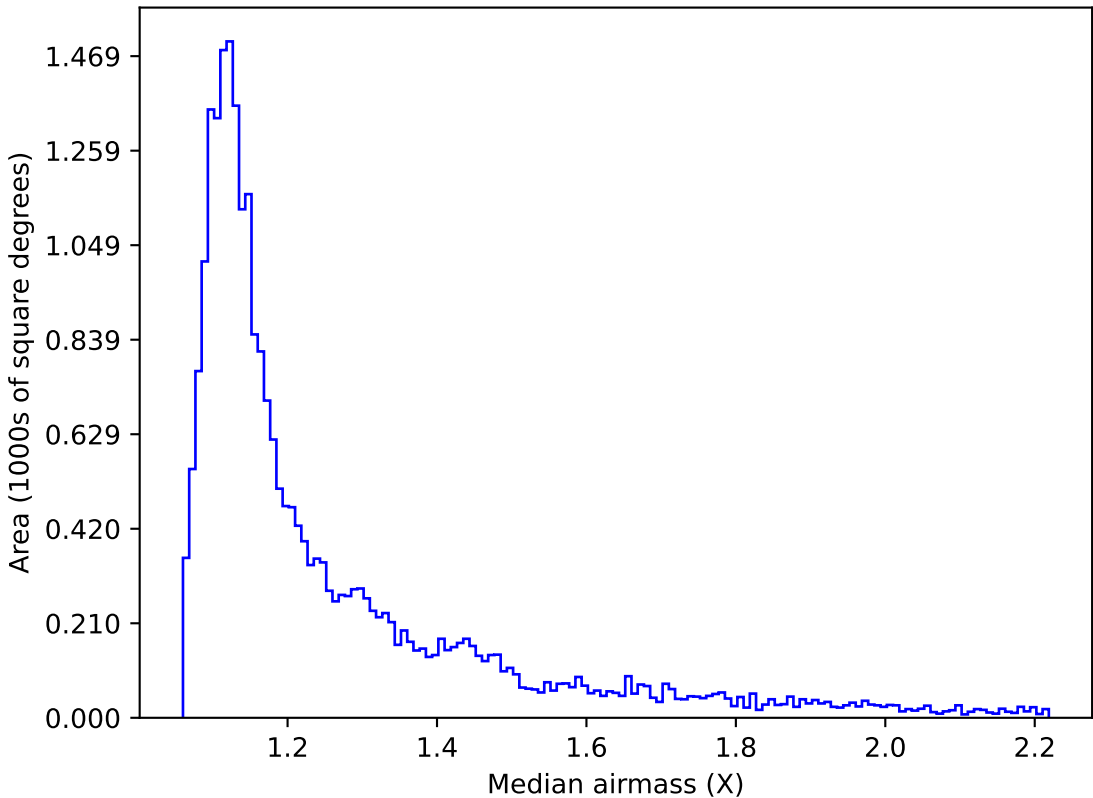
too_elab_r128_d2_griz_v3.4_10yrs Yr 1 z band: Median airmass
