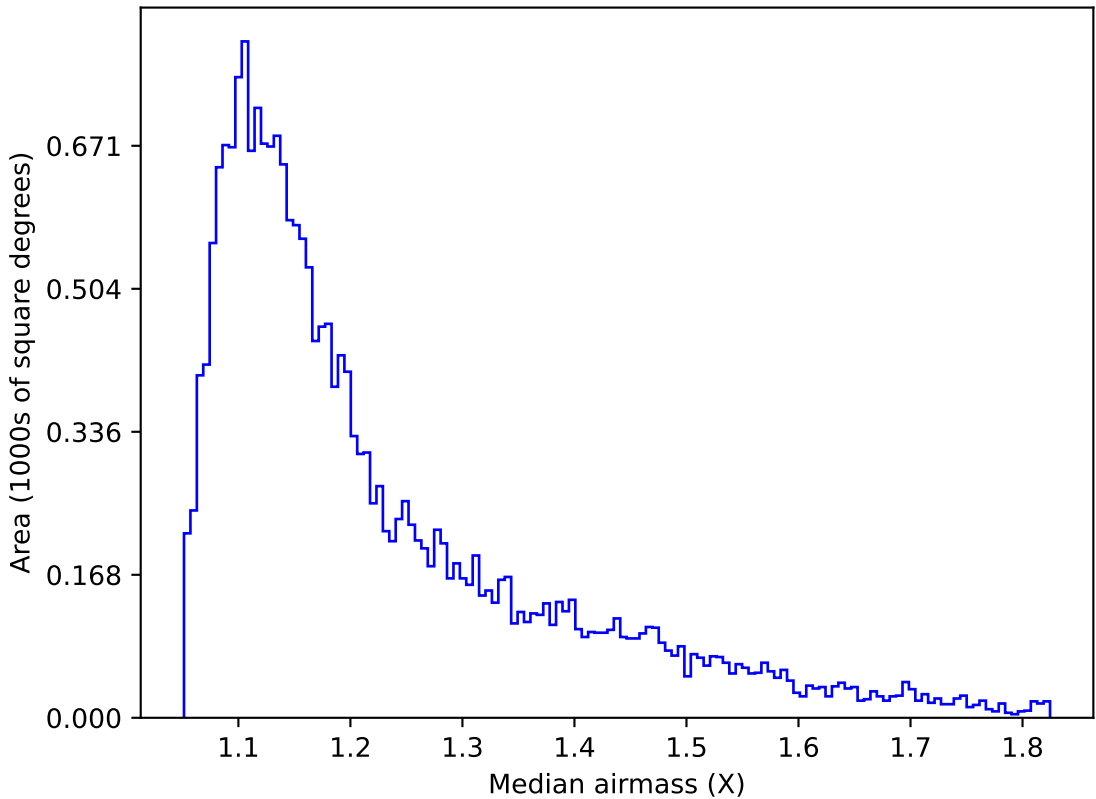
too_elab_r128_d2_griz_v3.4_10yrs Yr 1 u band: Median airmass
