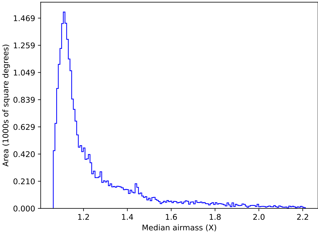
too_elab_r128_d2_griz_v3.4_10yrs Yr 1 i band: Median airmass
