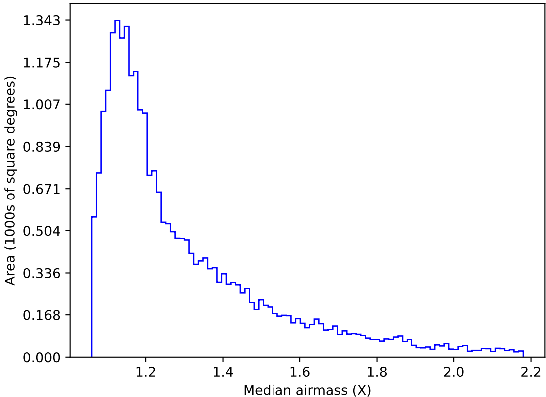
too_elab_r128_d2_griz_v3.4_10yrs Yr 1 g band: Median airmass
