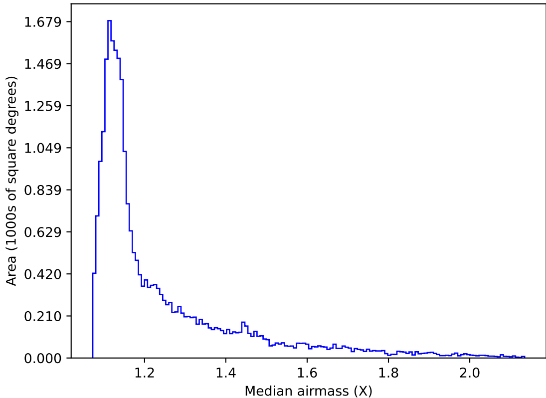
too_elab_r128_d2_griz_v3.4_10yrs Yr 1 all bands: Median airmass
