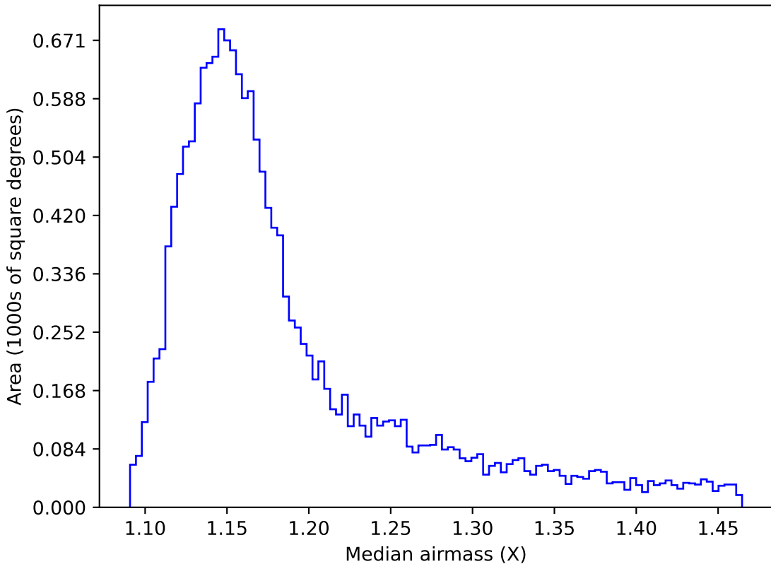
too_elab_r128_d2_griz_v3.4_10yrs WFD z band: Median airmass
