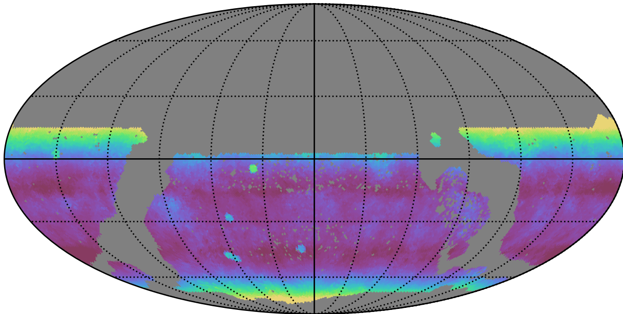
too_elab_r128_d2_griz_v3.4_10yrs WFD y band: Median airmass
