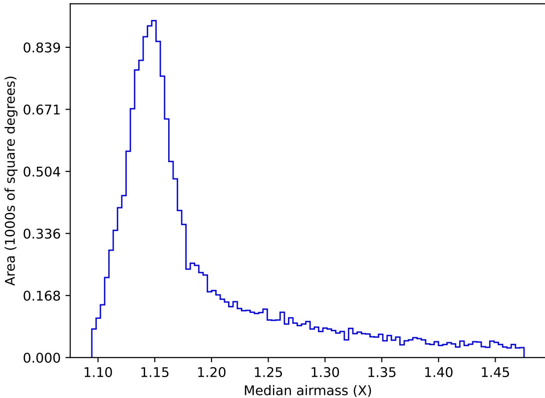
too_elab_r128_d2_griz_v3.4_10yrs WFD y band: Median airmass
