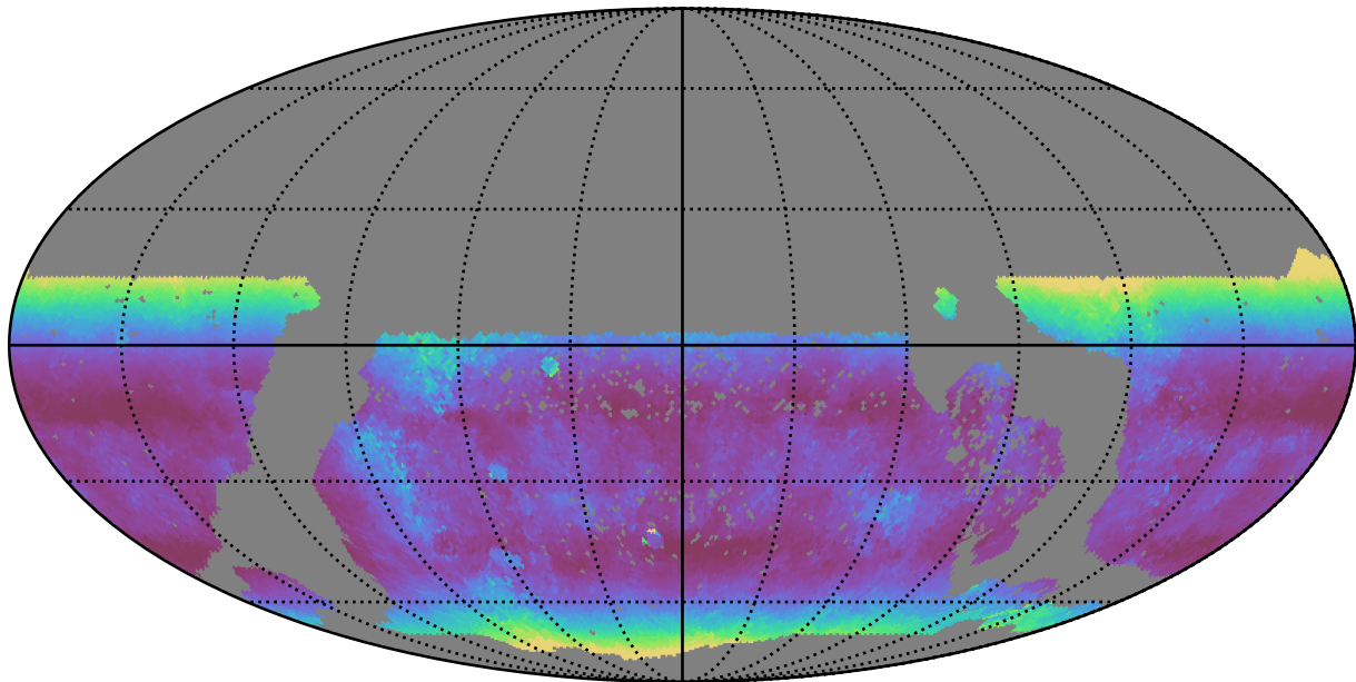
too_elab_r128_d2_griz_v3.4_10yrs WFD u band: Median airmass
