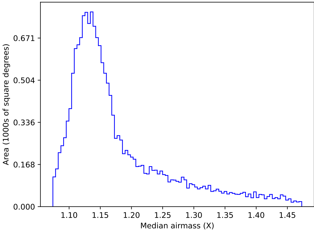
too_elab_r128_d2_griz_v3.4_10yrs WFD u band: Median airmass
