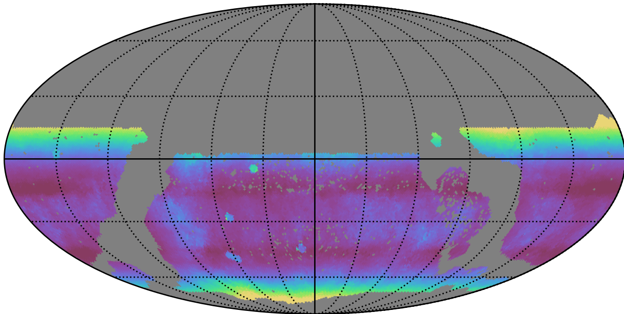
too_elab_r128_d2_griz_v3.4_10yrs WFD r band: Median airmass
