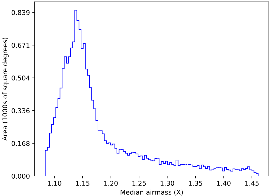
too_elab_r128_d2_griz_v3.4_10yrs WFD i band: Median airmass
