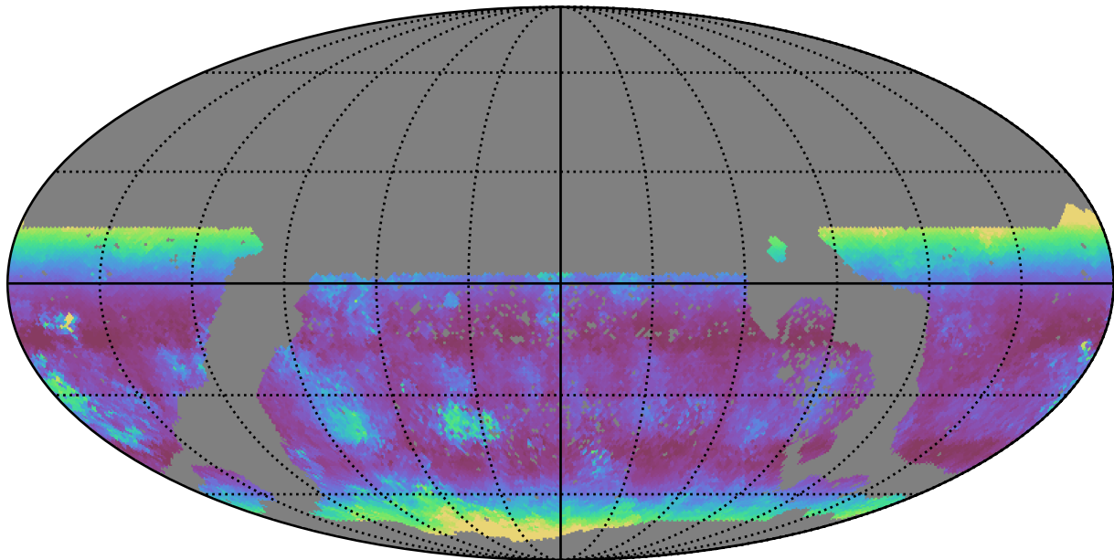
too_elab_r128_d2_griz_v3.4_10yrs WFD g band: Median airmass
