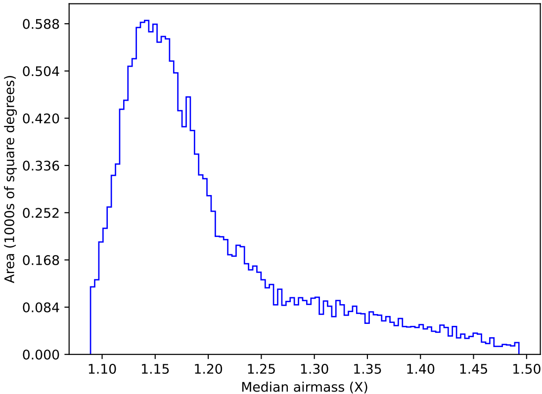
too_elab_r128_d2_griz_v3.4_10yrs WFD g band: Median airmass
