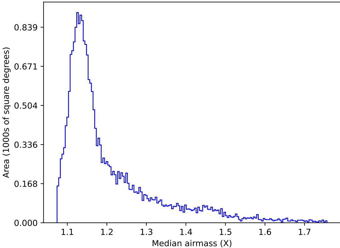
too_elab_r128_d2_griz_v3.4_10yrs All sky u band: Median airmass
