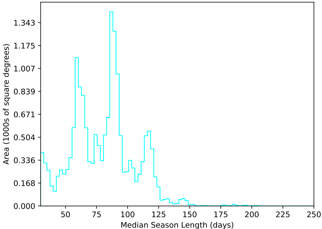
too_elab_r128_d2_griz_v3.4_10yrs WFD u band: Median Season Length
