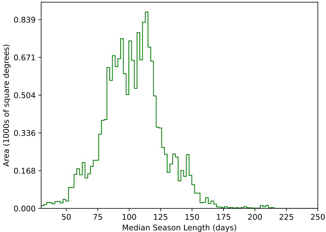
too_elab_r128_d2_griz_v3.4_10yrs WFD g band: Median Season Length
