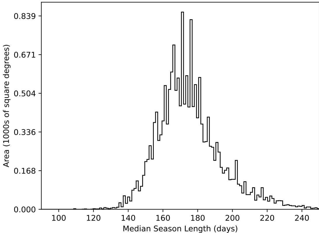
too_elab_r128_d2_griz_v3.4_10yrs WFD all bands: Median Season Length
