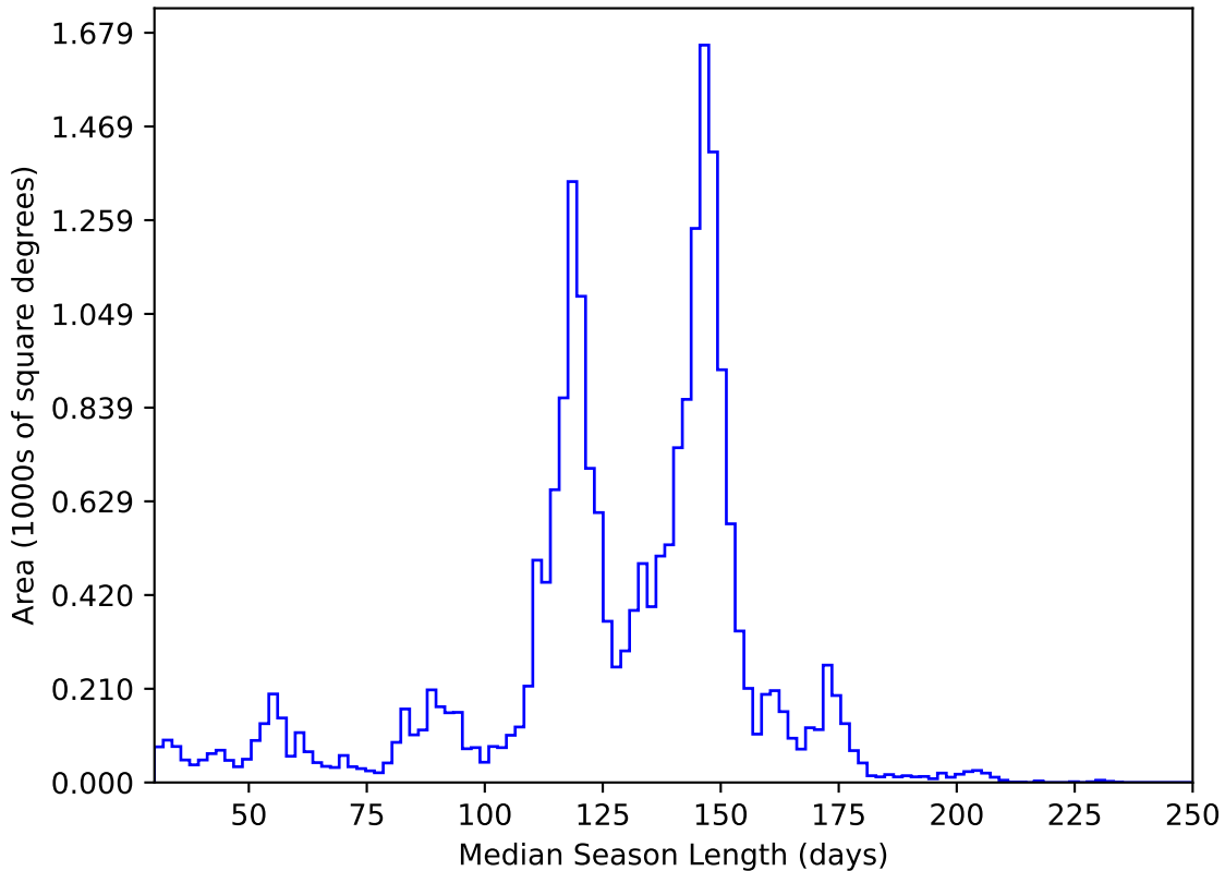
too_elab_r128_d2_griz_v3.4_10yrs All sky y band: Median Season Length
