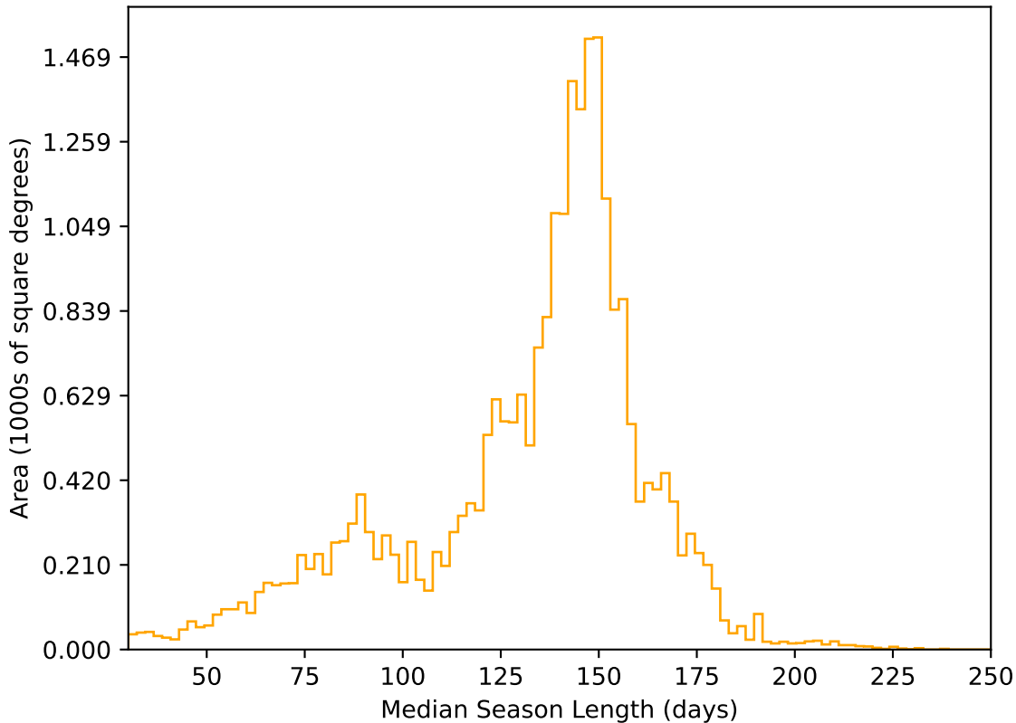
too_elab_r128_d2_griz_v3.4_10yrs All sky r band: Median Season Length
