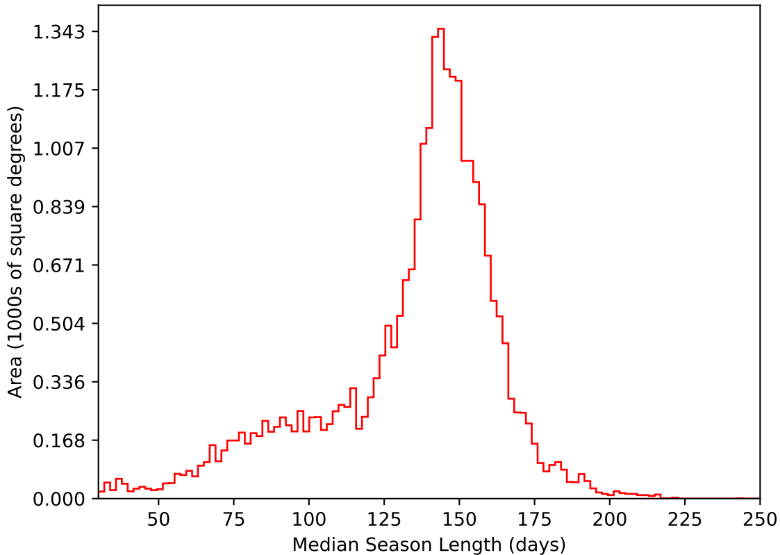
too_elab_r128_d2_griz_v3.4_10yrs All sky i band: Median Season Length
