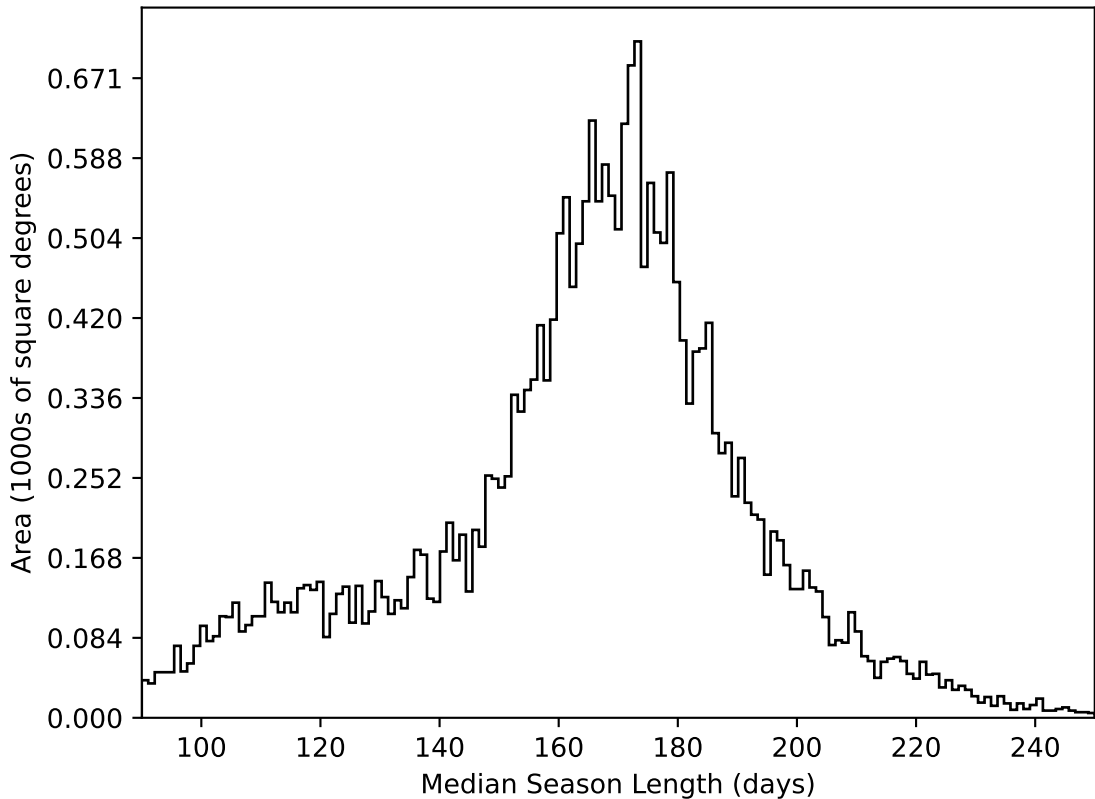
too_elab_r128_d2_griz_v3.4_10yrs All sky all bands: Median Season Length
