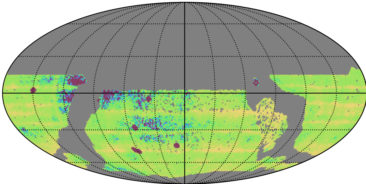
too_elab_r128_d2_griz_v3.4_10yrs WFD: Median Intra-Night Gap
