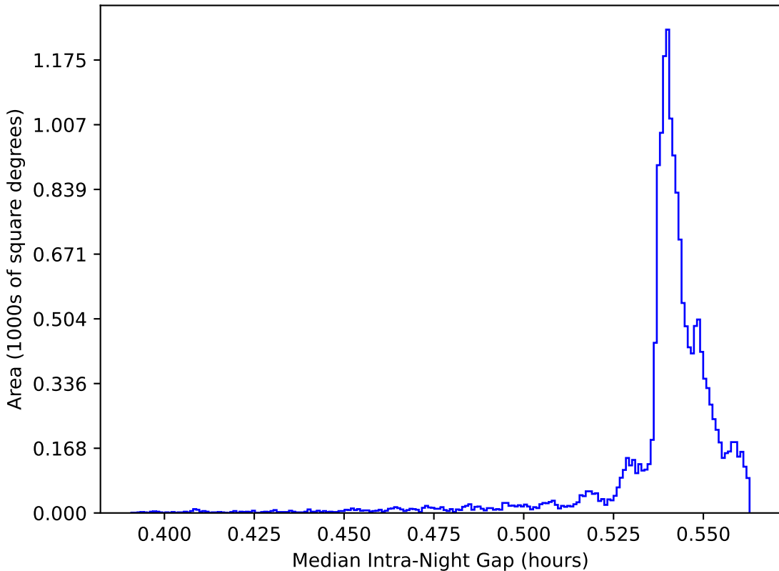
too_elab_r128_d2_griz_v3.4_10yrs WFD: Median Intra-Night Gap
