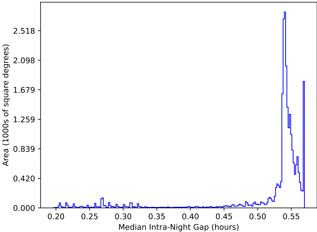
too_elab_r128_d2_griz_v3.4_10yrs All sky: Median Intra-Night Gap
