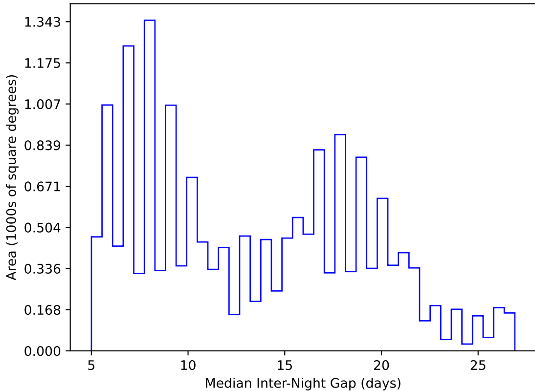
too_elab_r128_d2_griz_v3.4_10yrs WFD y band: Median Inter-Night Gap
