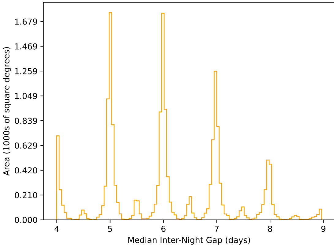
too_elab_r128_d2_griz_v3.4_10yrs WFD r band: Median Inter-Night Gap
