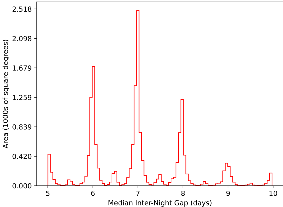
too_elab_r128_d2_griz_v3.4_10yrs WFD i band: Median Inter-Night Gap
