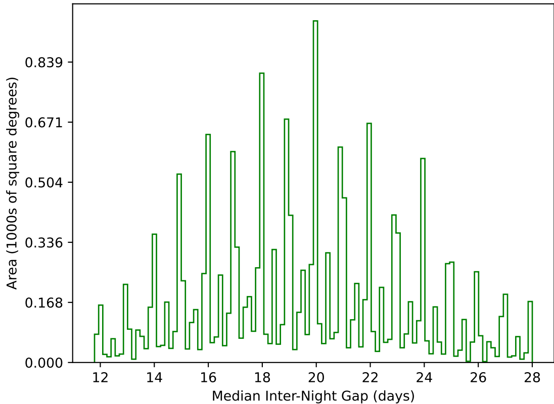
too_elab_r128_d2_griz_v3.4_10yrs WFD g band: Median Inter-Night Gap
