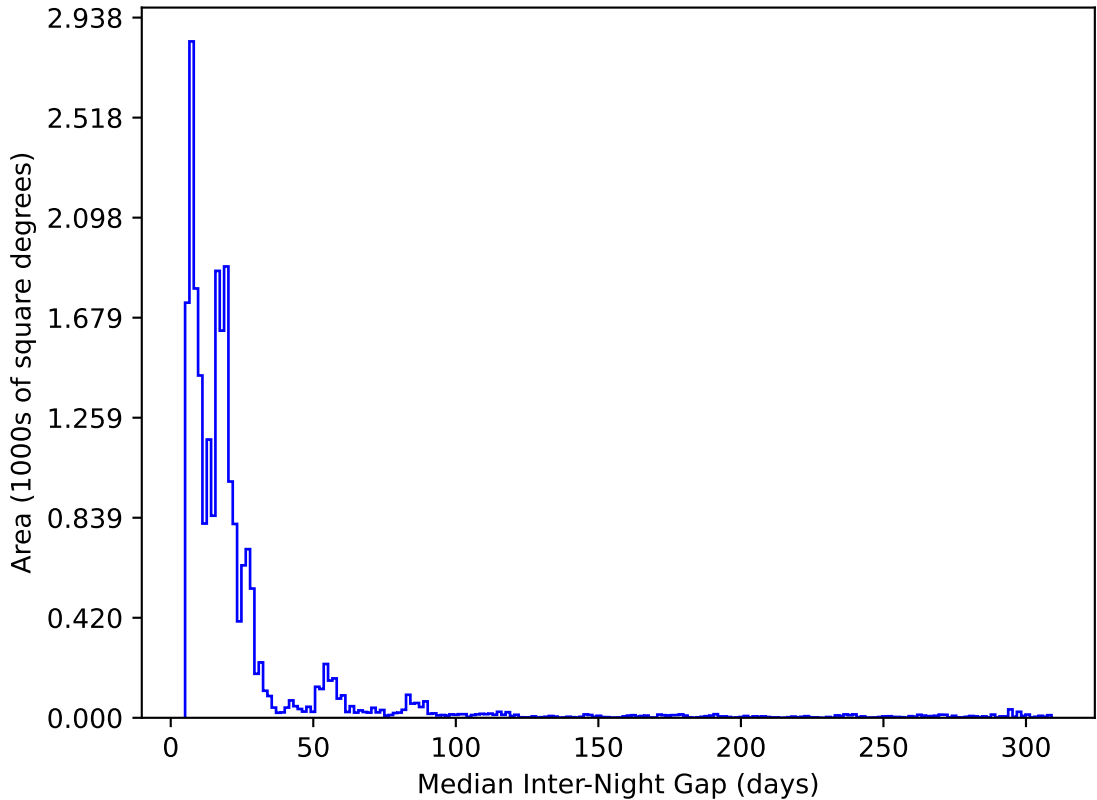
too_elab_r128_d2_griz_v3.4_10yrs All sky y band: Median Inter-Night Gap
