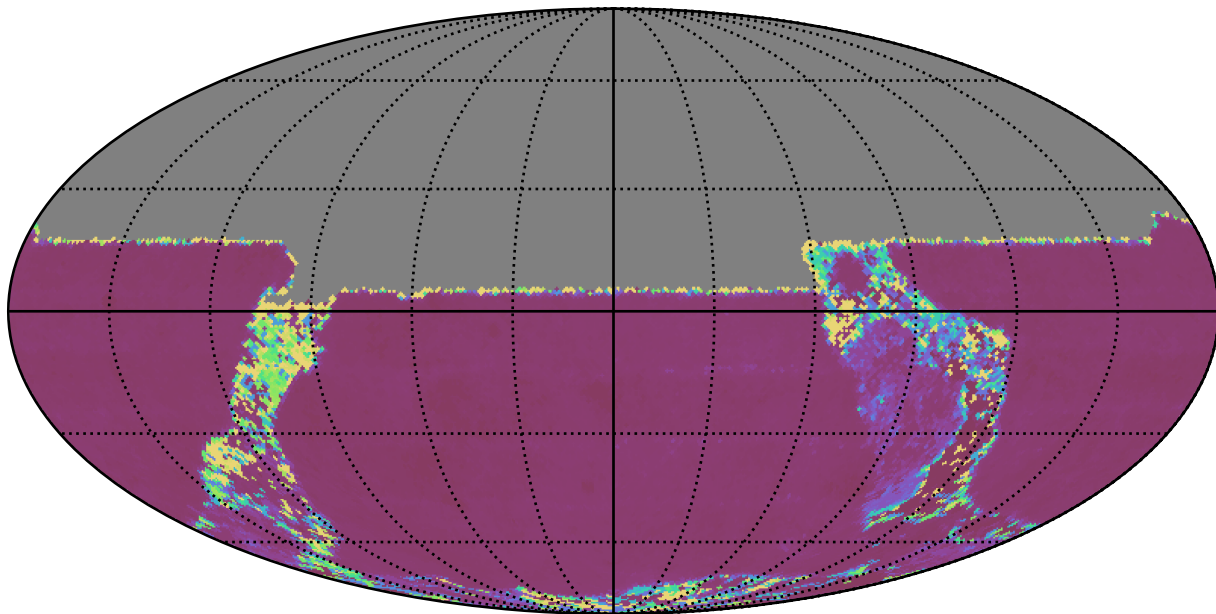
too_elab_r128_d2_griz_v3.4_10yrs All sky u band: Median Inter-Night Gap
