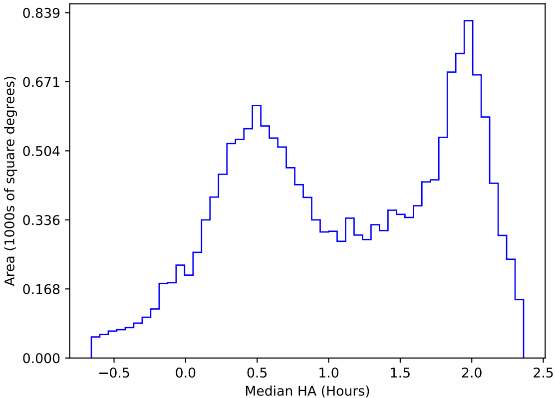
too_elab_r128_d2_griz_v3.4_10yrs WFD z band: Median HA
