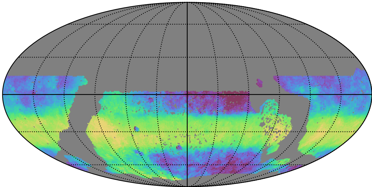
too_elab_r128_d2_griz_v3.4_10yrs WFD y band: Median HA
