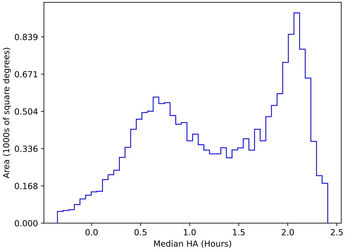
too_elab_r128_d2_griz_v3.4_10yrs WFD y band: Median HA
