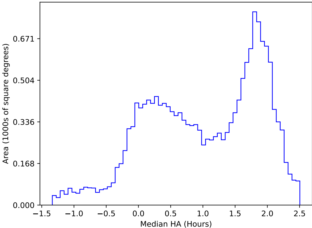
too_elab_r128_d2_griz_v3.4_10yrs WFD u band: Median HA
