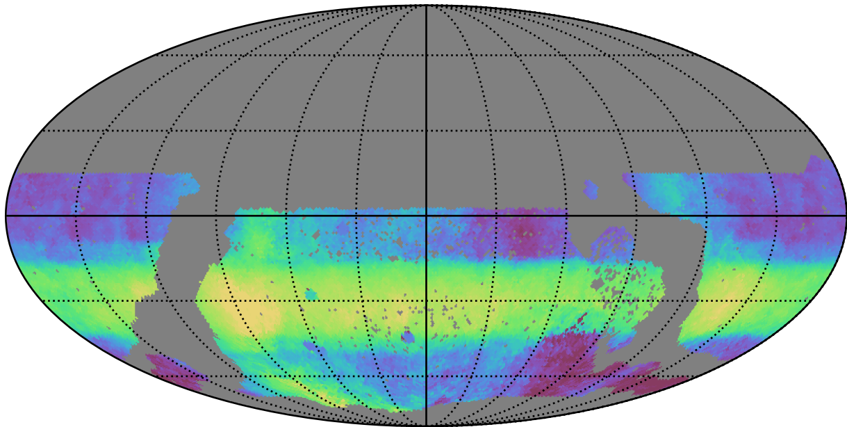
too_elab_r128_d2_griz_v3.4_10yrs WFD r band: Median HA
