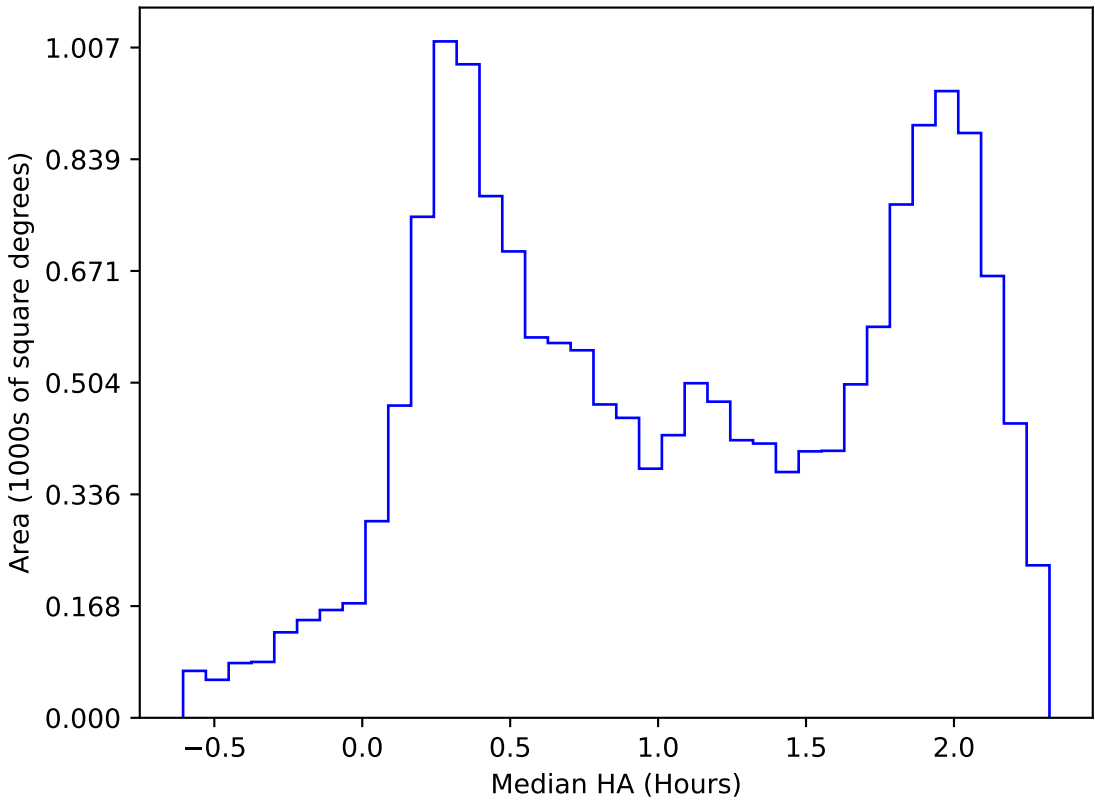
too_elab_r128_d2_griz_v3.4_10yrs WFD i band: Median HA
