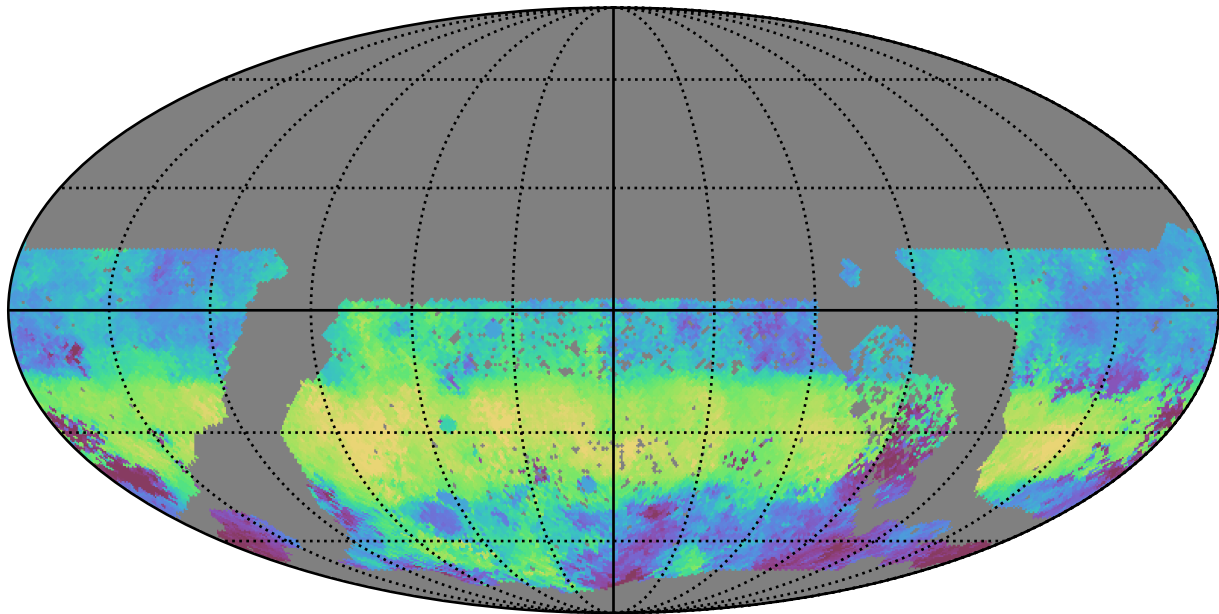
too_elab_r128_d2_griz_v3.4_10yrs WFD g band: Median HA
