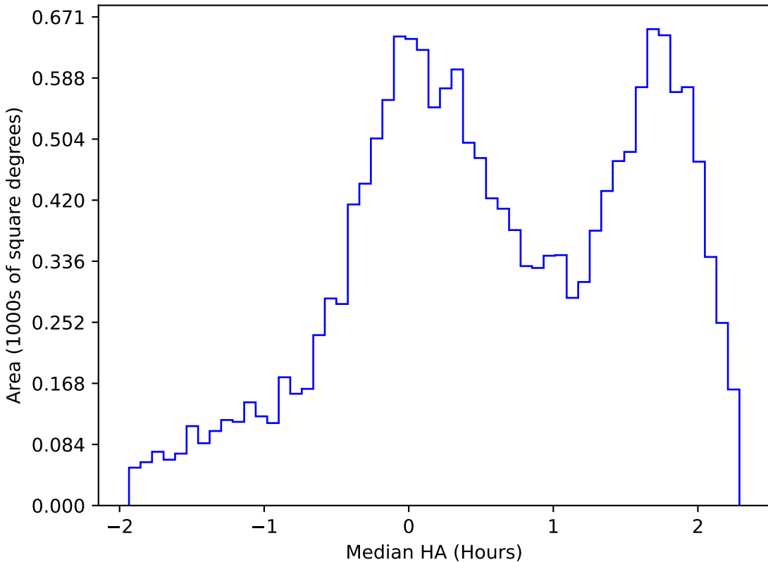
too_elab_r128_d2_griz_v3.4_10yrs WFD g band: Median HA
